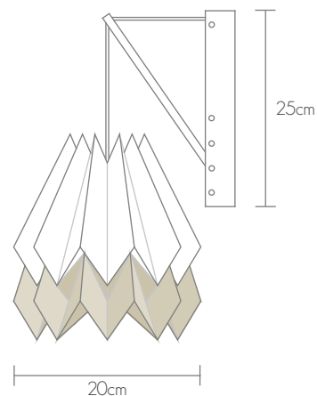
STRIPE WALL LAMPSHADE CANDEEIRO DE PAREDE c/ RISCAS ORI-WA-S-XX
